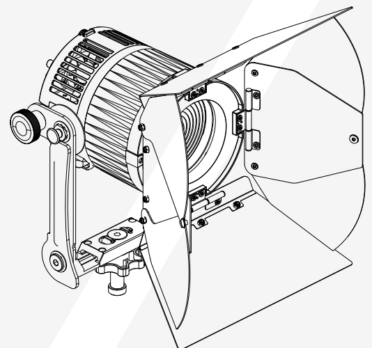
Barndoor attached to QuikBeam
